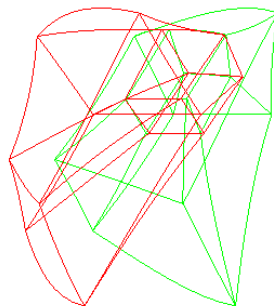
Fig. 10. Stereometric projections of 4D cube in a hyperboloid projective space
