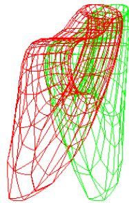
Fig. 11. Stereometric projections of 4D surface in a hyperboloid projective space f(x,y,z,w) = \{\cos(x), \sin(x), \cos(y)\sqrt{y^2}, \sin(y)\}
