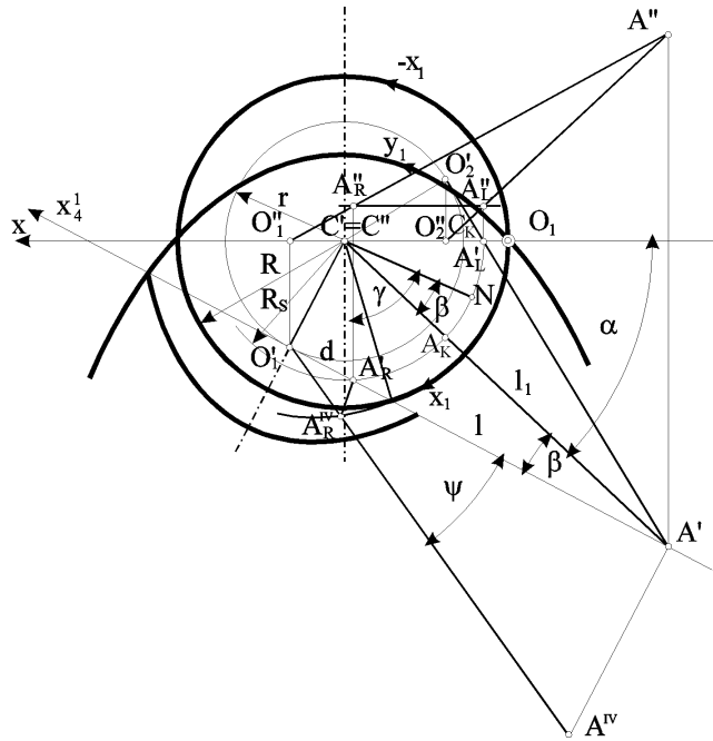
Fig. 4. Graphical representation of the mathematical model for stereometric projection in a paraboloid projective space
