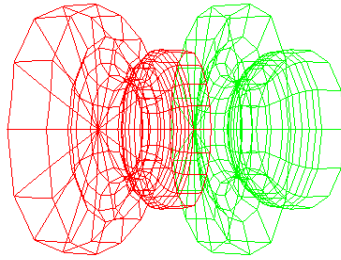
Fig. 7. Stereometric projections of 3D object in a hyperboloid projective space
