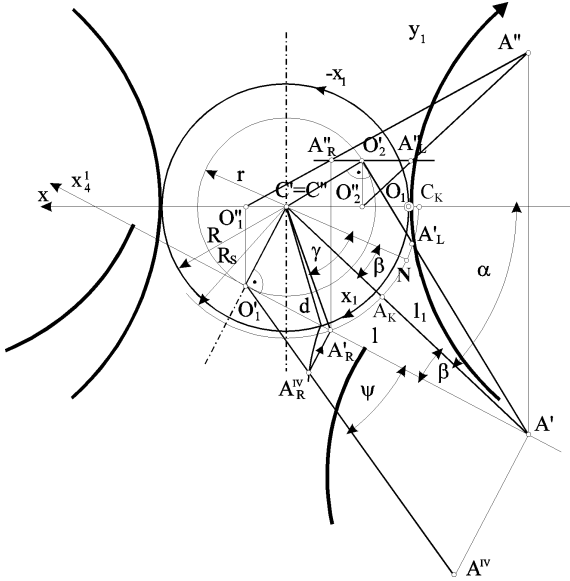
Fig. 2. Graphical representation of the mathematical model for stereometric projections in a hyperboloid projective space
