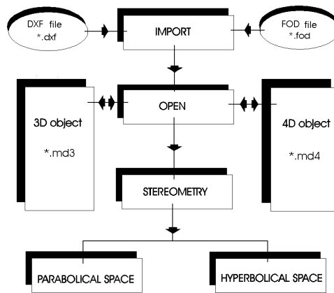
Fig. 5. Block diagram of algorithm for developing of stereometric projections in a hyperboloid and paraboloid projective space
