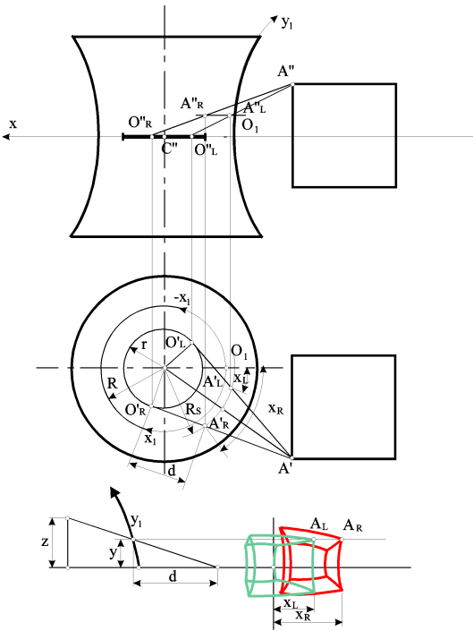
Fig. 1. Method for developing stereometric projections of a cube in a hyperboloid space
