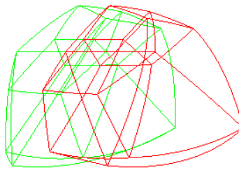
Fig. 12. Stereometric projections of 4D cube in a paraboloid projective space.
