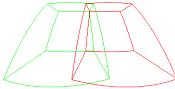
Fig. 8. Stereometric projections of a cube in a paraboloid projective space
