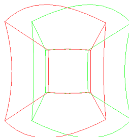
Fig. 6. Stereometric projections of a cube in a hyperboloid projective space
