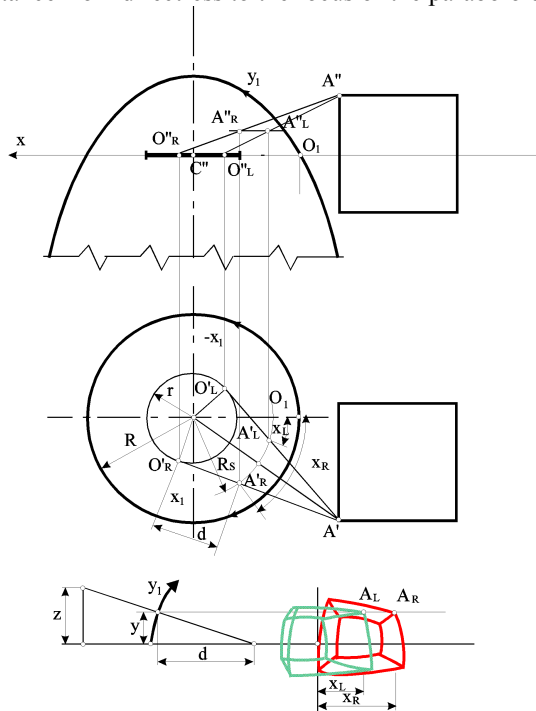
Fig. 3. Method for developing stereometric projection of a cube in a paraboloid projective space
