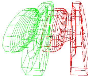
Fig. 9. Sterometric projections of 3D object in a paraboloid projective space
