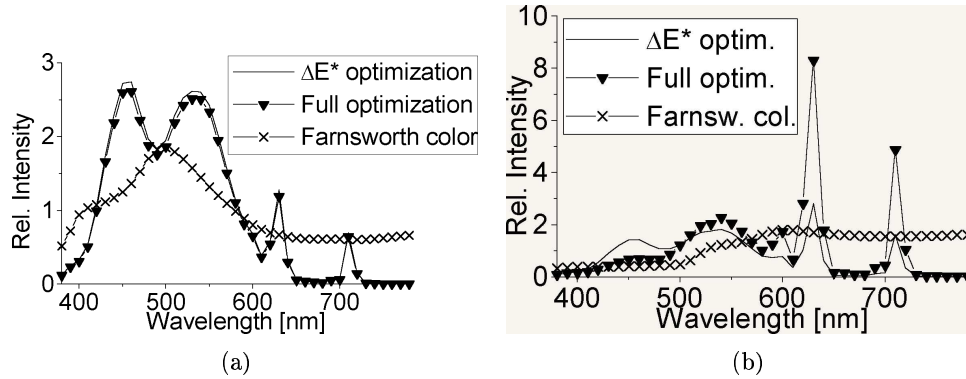
Fig. 4. The reflexive spectrum of Fransworth cap 15 (a) and cap 45 (b) in comparison with partially and totally optimized (R, G, B)_{DAC} emission.
