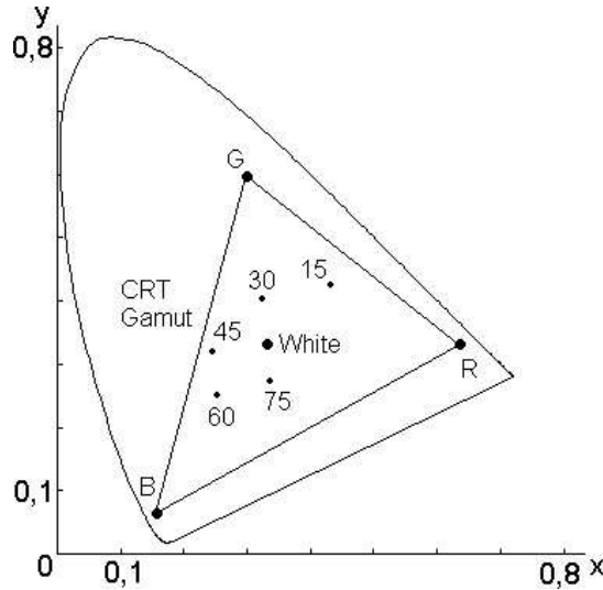
Fig. 3. Color presentation capability of a CRT display containing P22 phosphorus, and the ellipse of the Farnsworth 100 Hue test's color.
