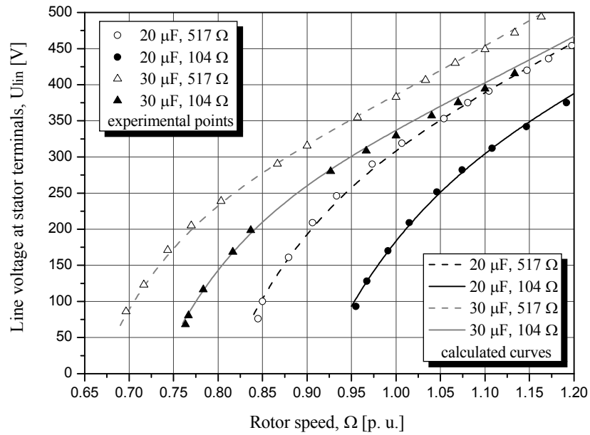
Fig. 4. Line voltage U_{lin} versus \Omega , for R_L = \text{const.} , C = \text{const.}
