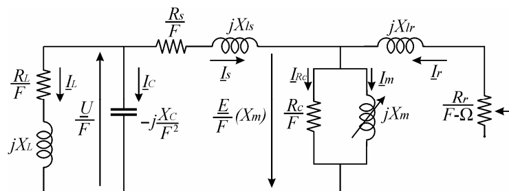
Fig. 1. Per-phase equivalent circuit of a three-phase SEIG
