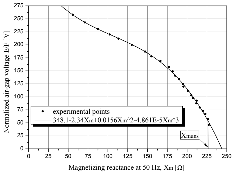
Fig. 2. Normalized air-gap voltage versus X_m
