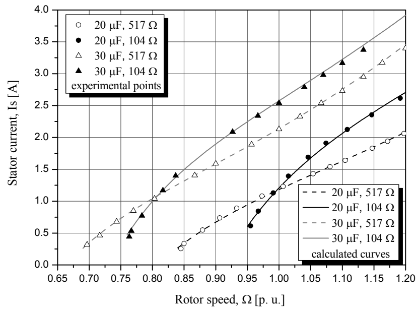
Fig. 5. Stator current I_s versus \Omega , for R_L = \text{const.} , C = \text{const.}
