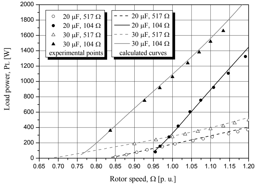
Fig. 6. Load power P_L versus \Omega , for R_L = \text{const.} , C = \text{const.}
